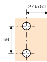
Fixed part
