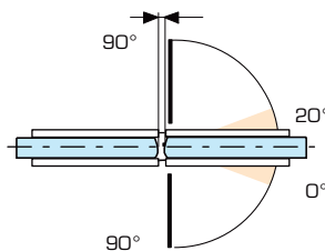
Glass/Glass 2 mm
