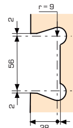
Mobile part
